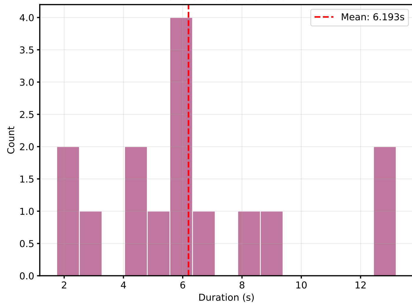
Red Step 0-250 Reverse Event Duration
